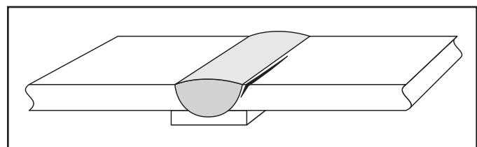
Figure 9-5 Heat affected zone cracking
