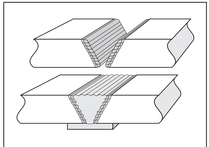
Figure 9-2 Buttering layers
