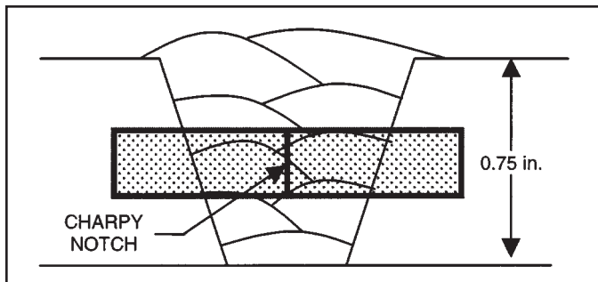
Figure 6-8 Typical CVN specimen location
