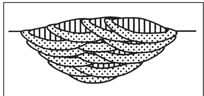
Figure 6-4 Grain refinement for flat weld beads
