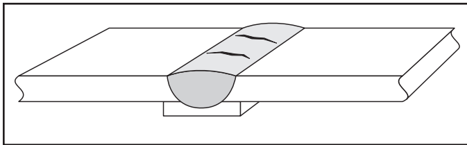
Figure 9-6 Transverse cracking
