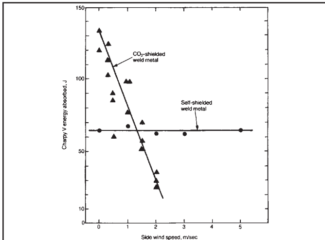
Figure 3-4b Comparison of the effect of side wind speed on Charpy V-notch impact toughness of: (a) CO 2 -shielded at room temperature and (b) self shielded ferritic steel weld metals at 0°C.
