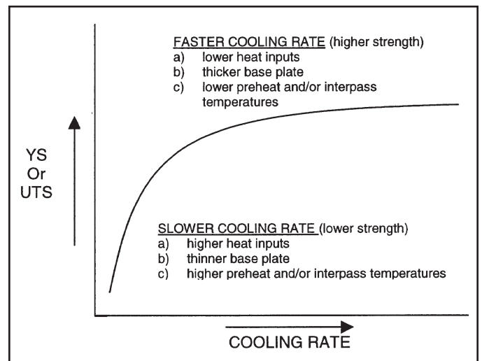
Figure 6-6 Strength related to cooling rate
