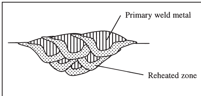
Figure 6-3 Grain refinement in multiple pass weld
