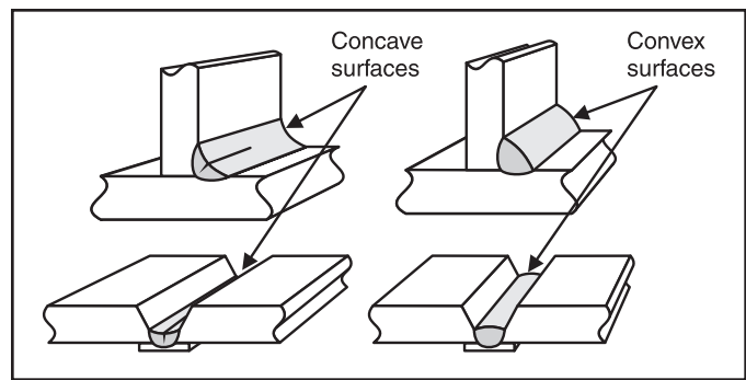
Figure 9-4 Surface profile induced cracking
