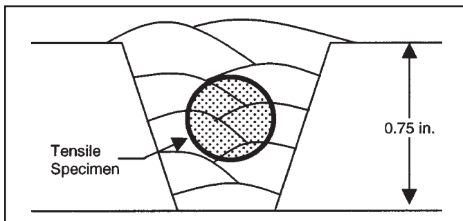
Figure 6-5 Typical tensile specimen location
