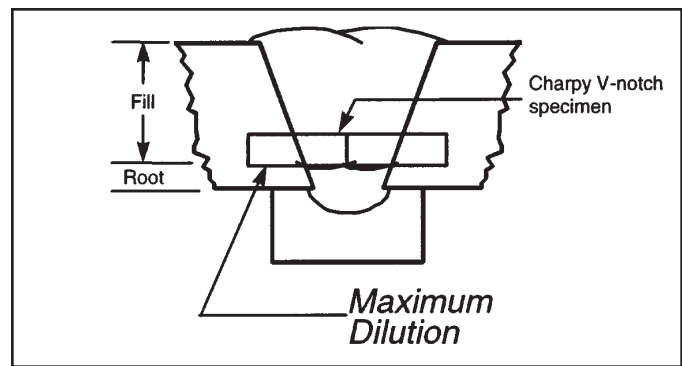
Figure 6-9 Locations of CVN test specimens
