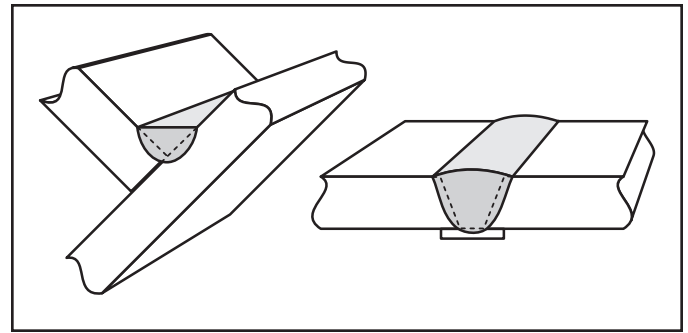
Figure 3-1 Joints requiring substantial fill
