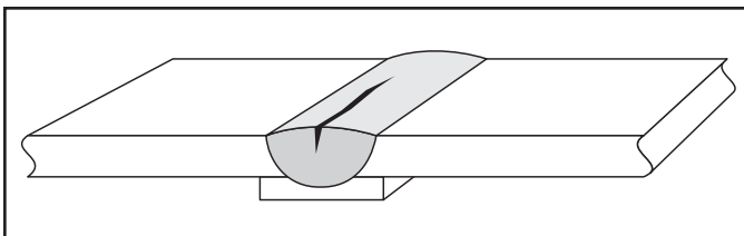
Figure 9-1 Centerline cracking
