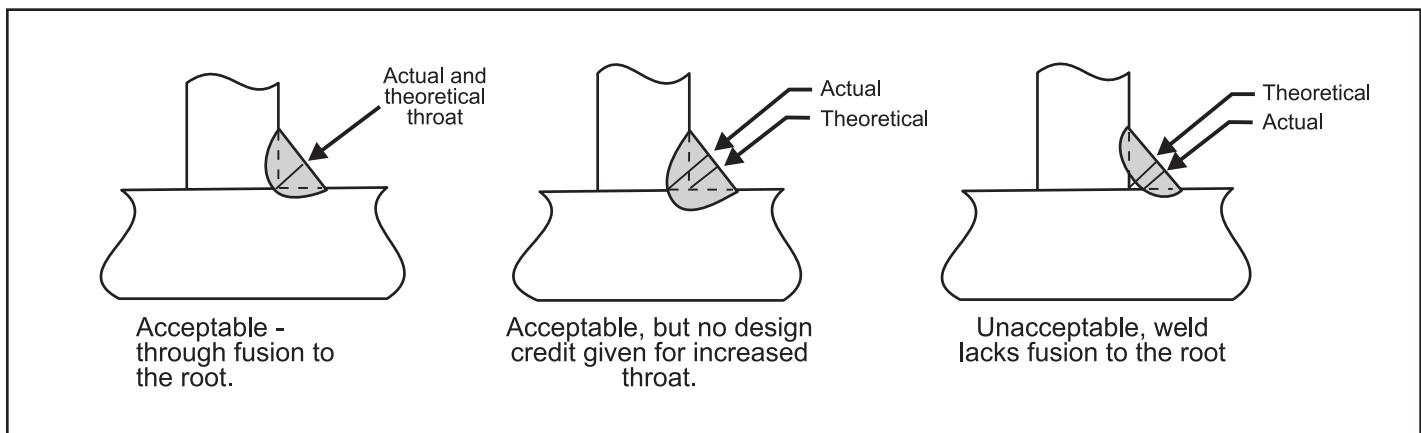
Figure 3-3 Fillet weld requirements
