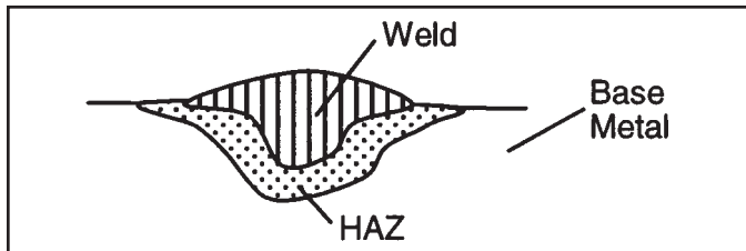
Figure 6-2 Three zones created by welding
