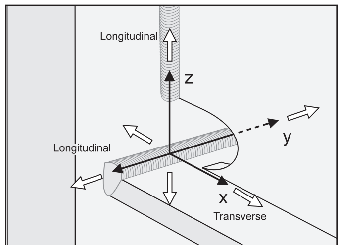
Figure 6-1 Minimization of triaxial stress at the weld access hole
