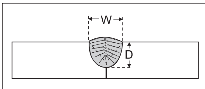
Figure 9-3 Bead shape induced cracking
