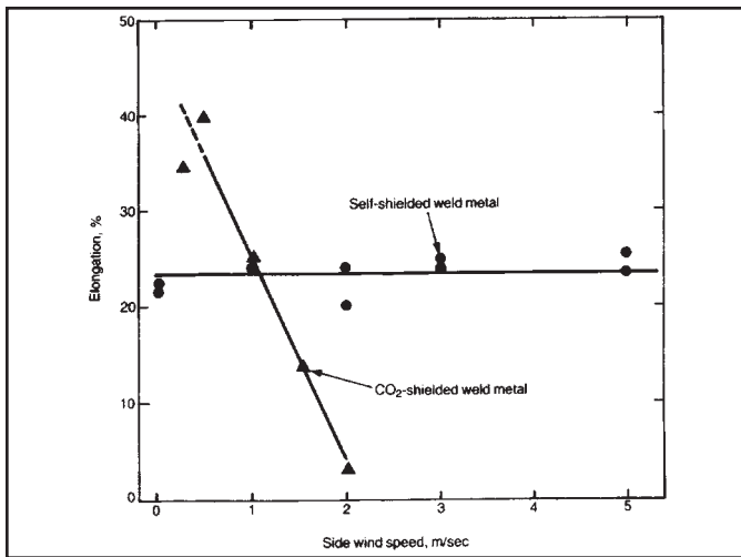
Figure 3-4a Comparison of the effect of side wind on tensile elongation of: (a) CO 2 -shielded and (b) self shielded ferritic steel weld metals.
