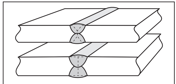
Figure 3-2 Joints requiring substantial penetration
