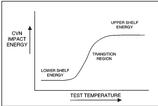
Figure 6-7 Schematic CVN transition curve
